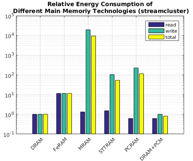
Fig. 4. This shows the energy consumption of different types of memory on the streamcluster workload relative to DRAM.
